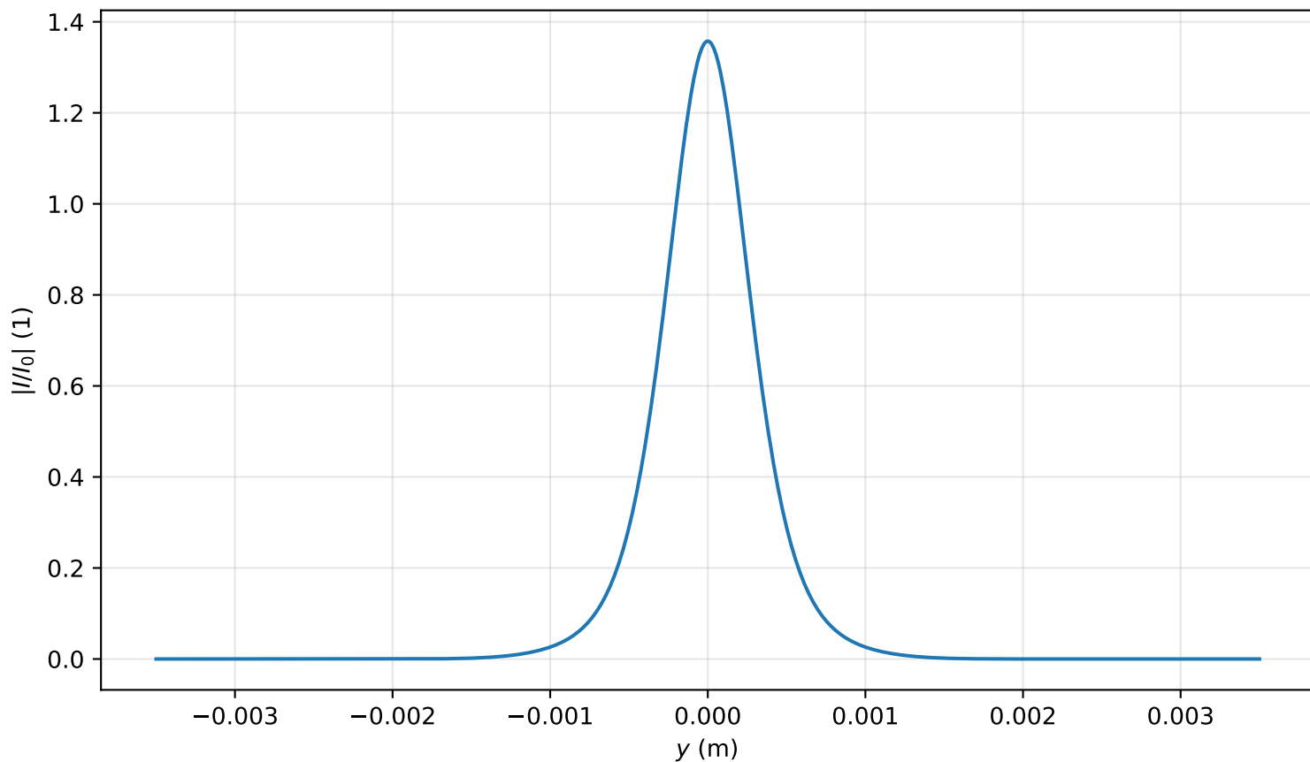
Intensity profile I(x=0, y, z=1.513)/I_0 , P_{in}=0.8P_{cr} , artificial time
